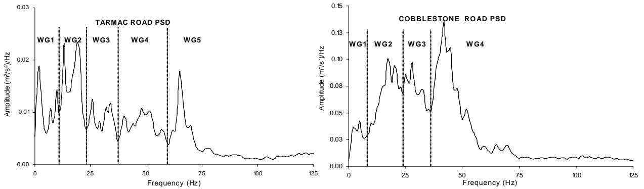
Figure 6. Power spectral densities of the steering acceleration time histories, showing the wavelet group boundaries chosen for use in the current study.
