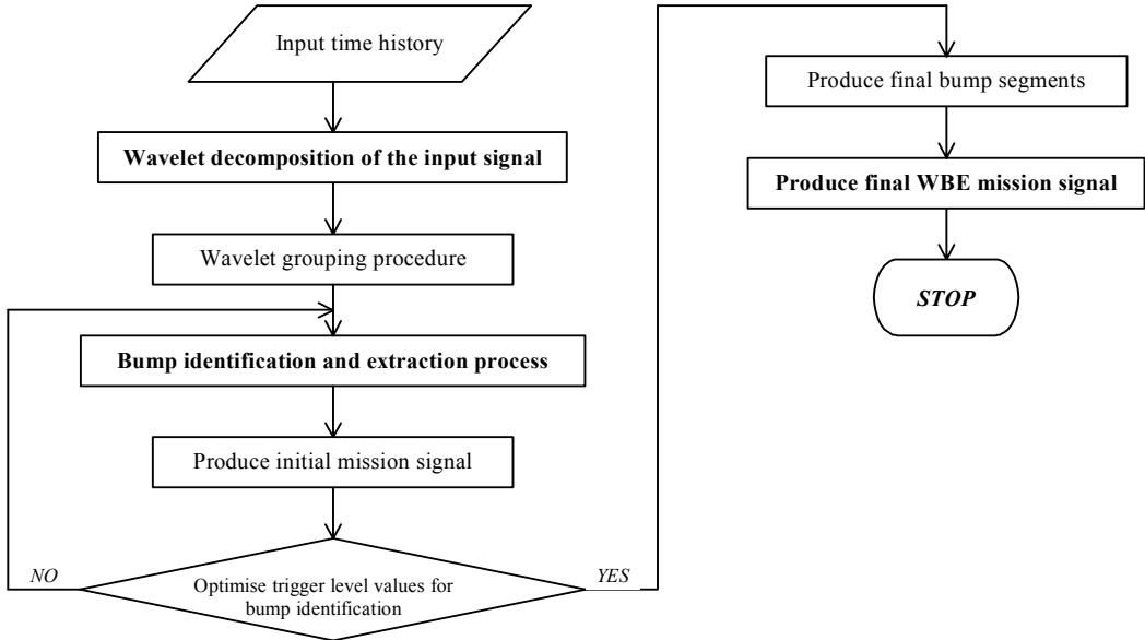
Fig. 1. Simplified flowchart of the WBE algorithm
