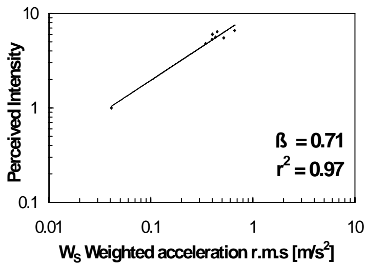
Figure 4) Mean Borg CR10 perceived intensities as a function of the unweighted, the W_h weighted and the W_s weighted r.m.s. acceleration amplitudes if the eight test stimuli ( \text{m/s}^2 ).
