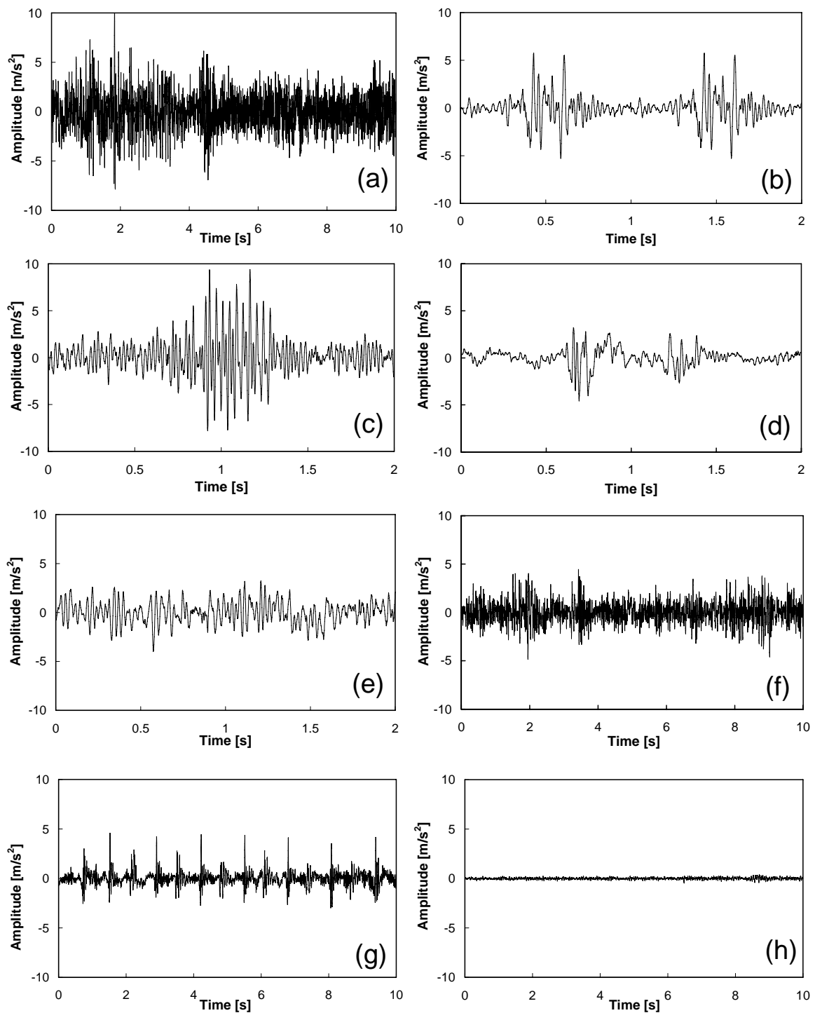
Figure 1) Steering wheel acceleration time histories used in the laboratory experiments: (a) country lane (vehicle speed 80 Km/h), (b) pothole (vehicle speed 60 Km/h), (c) rumble strip (vehicle speed 60 Km/h), (d) stone on road (vehicle speed 20 Km/h), (e) manhole cover (vehicle speed 60 Km/h), (f) city street (vehicle speed 50 Km/h), (g) expansion joints (vehicle speed 16 Km/h) and (h) motorway (vehicle speed 96 Km/h).
